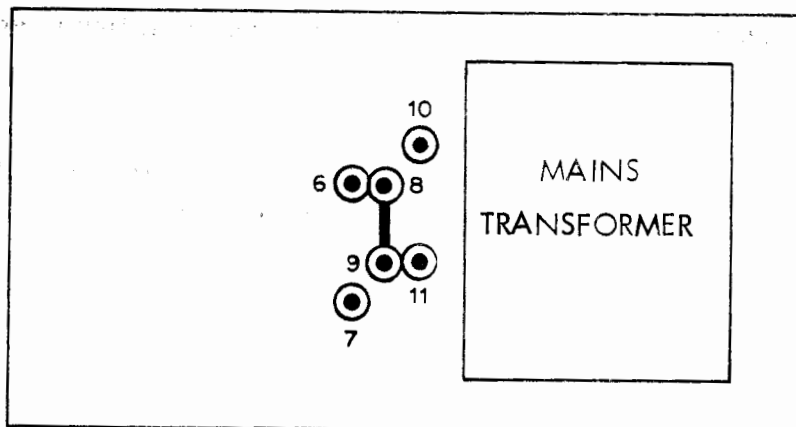
PCB LINK ARRANGEMENT FOR 190 - 270V 40/60Hz AC.
