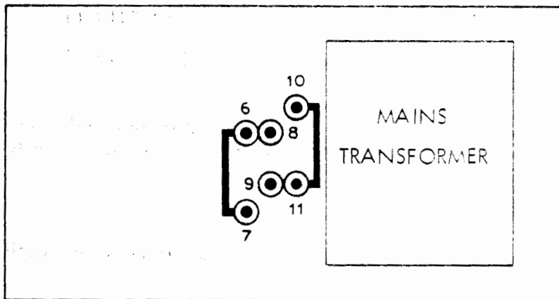
PCB LINK ARRANGEMENT FOR 105 - 125V 40/60Hz AC.
